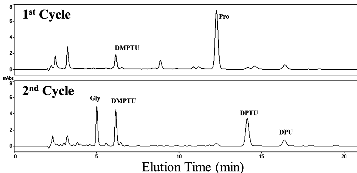
Figure 3. Peptide sequence analysis of peaks marked in Figure 2. Phenylthiohydantoin (PTH) amino acid elution profiles at the 1st and 2nd steps are shown. DMPTU: N -dimethyl- N' -phenylthiourea. DPTU: N,N' -diphenylthiourea. DPU: sym -diphenylurea.
